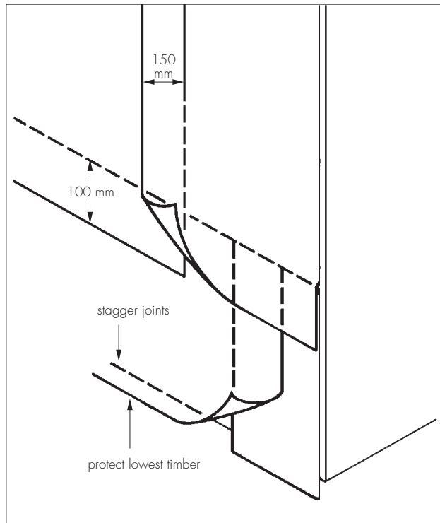
Figure 1 Membrane installation
