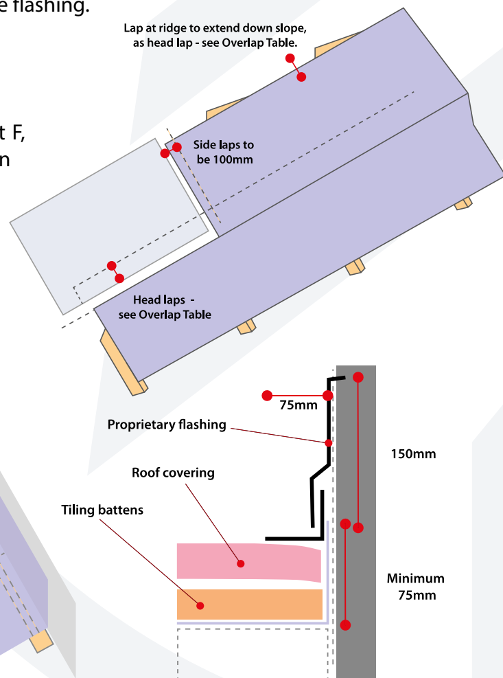
Figure 3 - Overlap Detail
