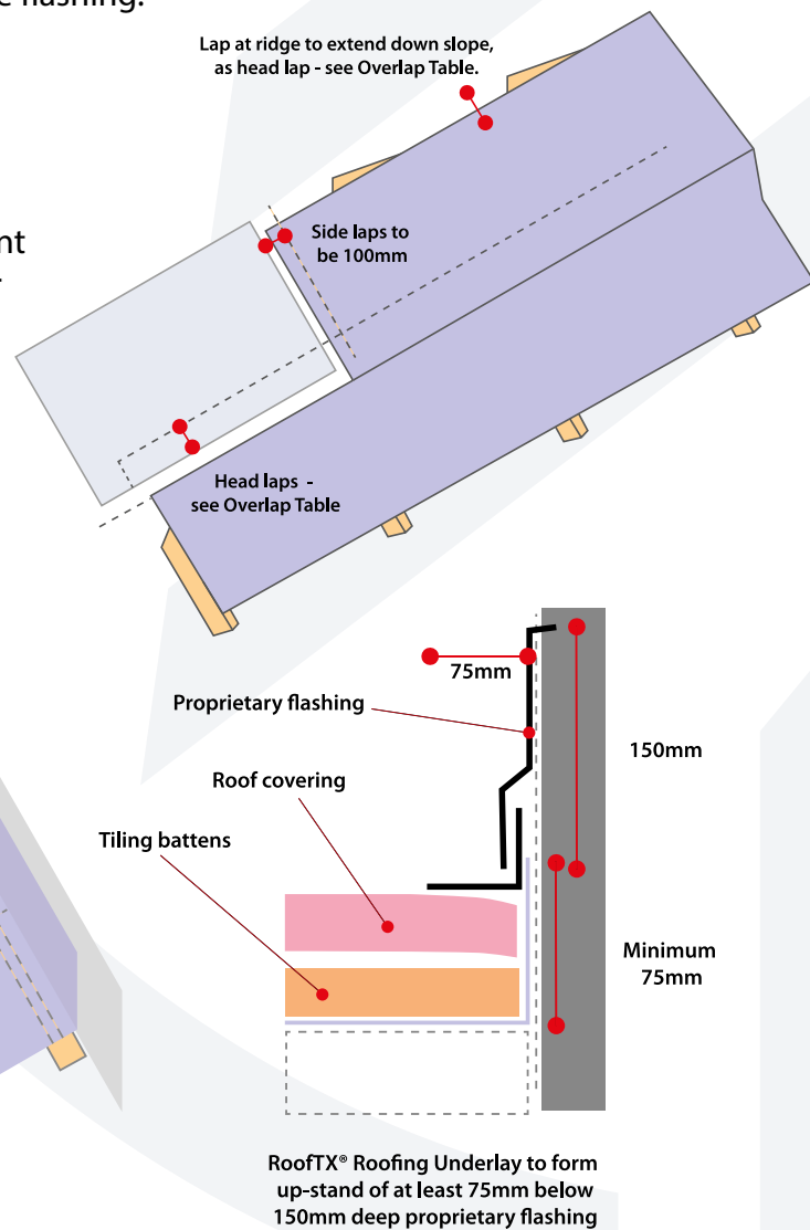
Figure 3 - Overlap Detail
